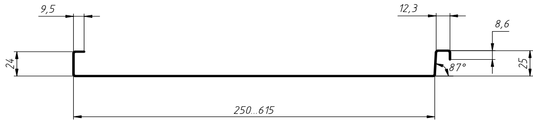
Profile drawing for standing seam roofing machine FM/F3
