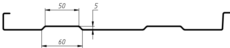
Drawing of the ribbed profile for standing seam roofing machine FM/F3
